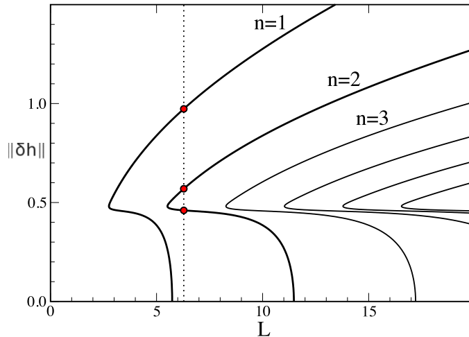
FIG. 19. The bifurcation diagram for contact angle \beta_0 = 2 for the simplified system without gravity ( B = 0 ) and without rotation ( \Omega = 0 ) but for an extended domain size L that is employed as the control parameter. The dotted vertical line indicates the value L = 2\pi that corresponds to our system in the chosen scaling. The various curves represent n -drop solutions upon the cylinder. The three crossings of branches and the vertical line represent one stable single-drop solution and two unstable double-drop solutions, which is consistent with the number of solution seen in Fig. 6 for B = 0 .
