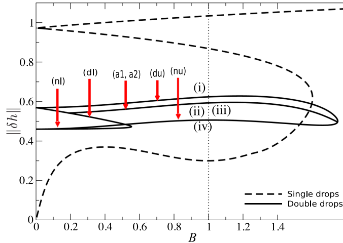
FIG. 6. Branches of steady profiles for \beta_0 = 2 . The L^2 -norms are given as functions of the Bond number B . The dashed lines represent single-drop solutions also present in Fig. 2(a) while the solid lines give the bifurcation structure of unstable double-drop solutions. There we distinguish symmetric drop (du, dl) and nucleation or hole (nu, nl) and asymmetric (a1, a2) solutions. Subscripts “u” and “l” refer to the respective upper and lower solution. The profiles at B = 1 (indicated by the vertical dotted line and marked by (i)–(iv)) are displayed in Fig. 7. We also note that only the branch that corresponds to pendent drop solutions is stable (the branch with the largest L^2 -norms). All the other branches are unstable.
