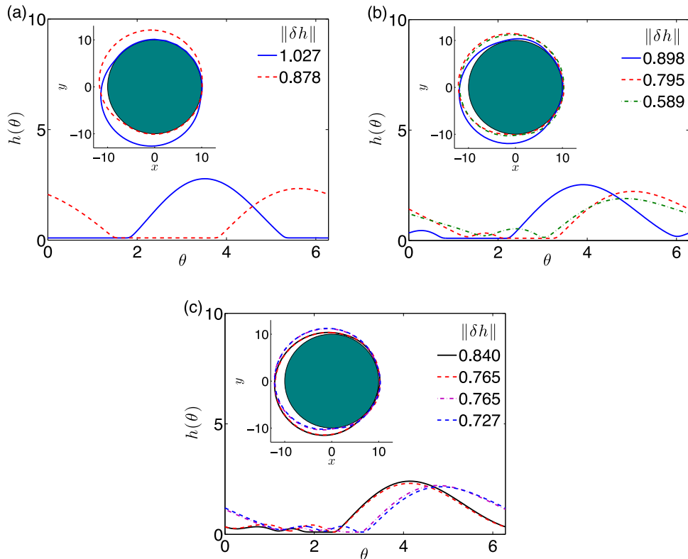
FIG. 5. Steady drop profiles on a horizontal cylinder for \Omega = 0.767 , \beta_0 = 2 and B = 1 , i.e., at the loci indicated by the vertical thin dashed line in Fig. 3(b). The individual panels give (a) single-, (b) double-, and (c) triple-drop solutions, with the L^2 -norms \|\delta h\| as given in the legends. The insets show the profiles on a cylinder assuming a radius R = 10 .
