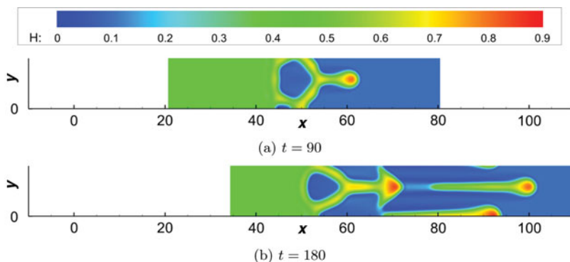
FIGURE 11. Height profile of a Type 2 ( \mathcal{N} = 10 ) flow down an inclined substrate at various times. Here the azimuthal substrate anchoring is ignored ( \eta = 0 ), and other parameters are given in Tables 1(a) and (b). The initial front position, x_f \approx 24 , and the initial condition is similar to Figure 4(a).
